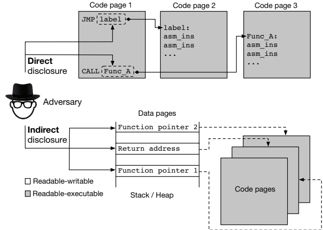
Figure 1: Direct and indirect memory disclosure.
