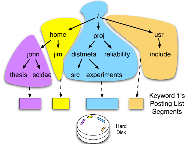
Fig. 1: Segment Partitioning. The namespace is broken into partitions that represent disjoint sub-trees. Each partition maintains posting list segments for keywords that occur within its sub-trees. Since each partition is relatively small, these segments can be kept sequential on-disk.
