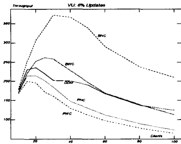
Figure 6: VU Experiment with 6% Update Jobs
