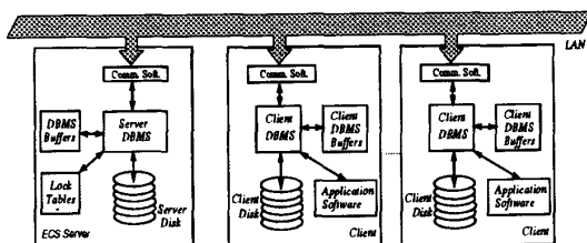
Figure 1: The ECS DBMS Architecture
