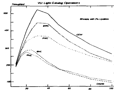
Figure 14: VU, Inexpensive Catalog Access
