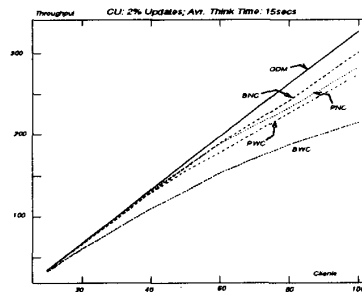
Figure 7: CU, 2% Updates, and Think Time
