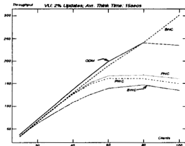
Figure 9: VU, 2% Updates, and Think Time
