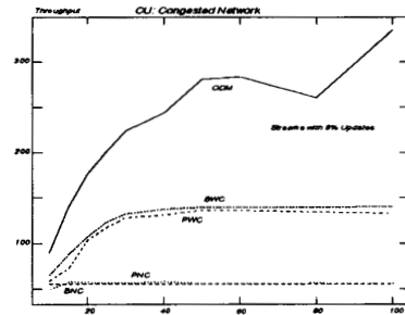
Figure 11: CU, Loaded Network, 8% Updates
