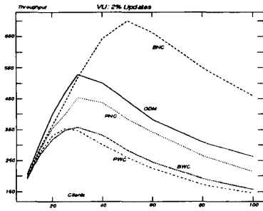
Figure 5: VU Experiment with 2% Update Jobs
