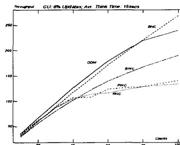
Figure 8: CU, 6% Updates, and Think Time
