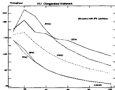
Figure 12: VU, Loaded Network, 8% Updates
