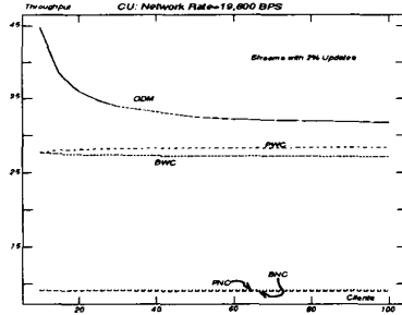
Figure 13: CU, Net. Rate 19,600 BPS
