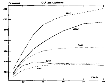
Figure 2: CU Experiment with 2% Update Jobs
