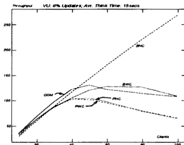
Figure 10: VU, 6% Updates, and Think Time
