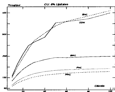
Figure 3: CU Experiment with 6% Update Jobs
