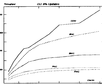
Figure 4: CU Experiment with 8% Update Jobs
