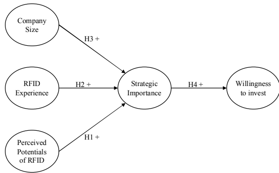
Figure 1: Research model
