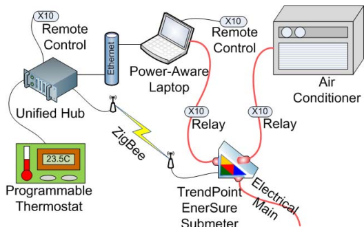
Figure 3. Test Bed
