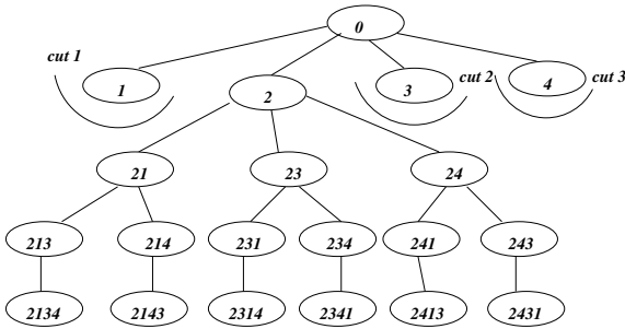
Figure 5. n = 4 , Branch and Bound Tree after Pruning
