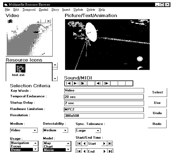
Figure 4: The Multimedia Resource Browser
