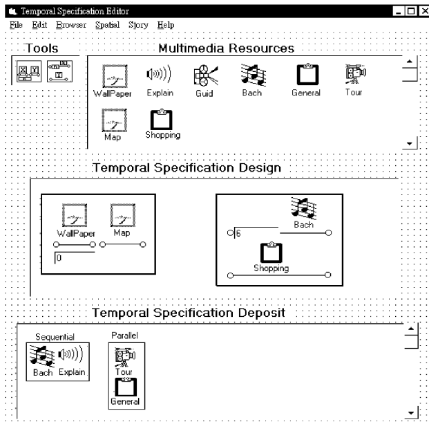
Figure 5: The Temporal Specification Editor
