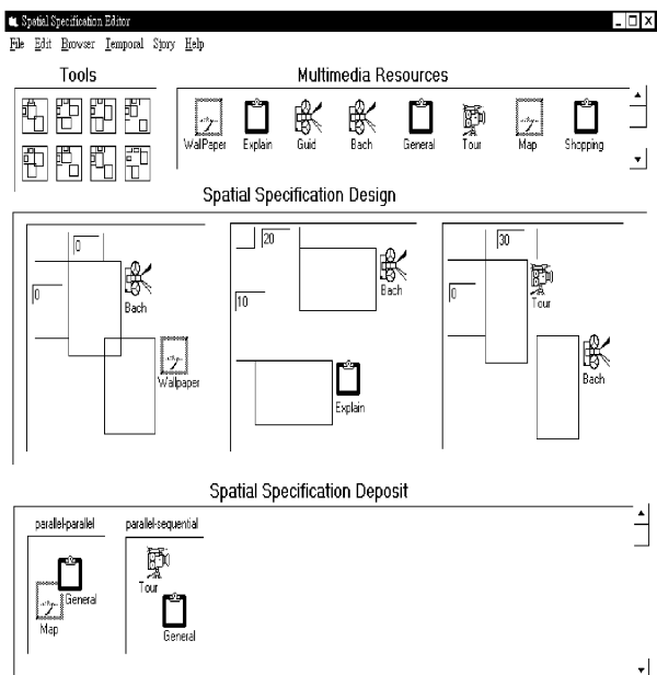
Figure 7: The Spatial Specification Editor
