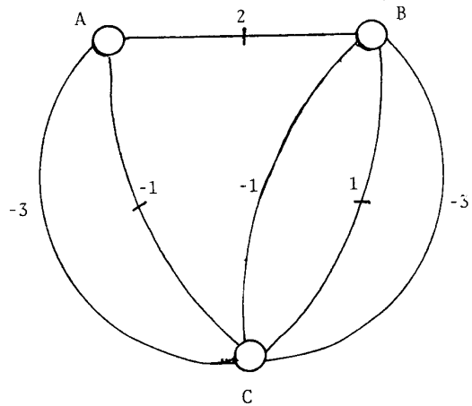
Fig. 9. Geometric dual of G
