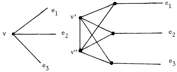
Fig. 7. The star substituting a vertex
