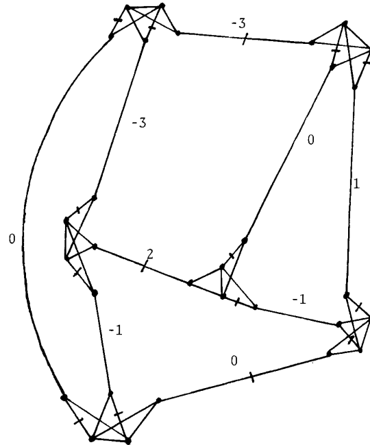
Fig. 7. The star substituting a vertex
