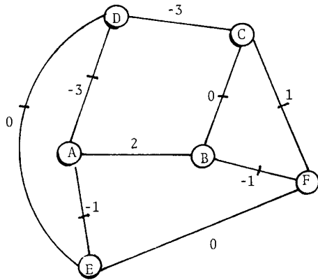
Fig. 5. Triangulation G_t of G
