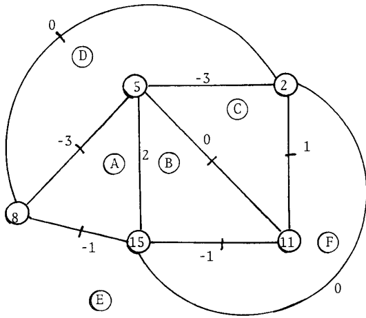
Fig. 4. Optimal layer assignment
