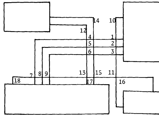
Fig. 1. Layout before layer assignment
