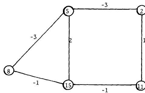
Fig. 3. Cluster graph G
