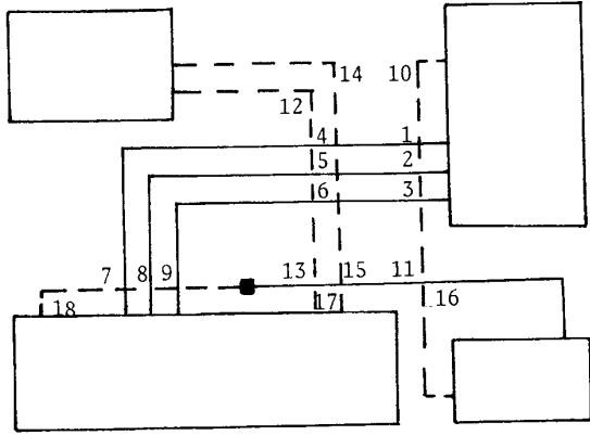
Fig. 4. Optimal layer assignment
