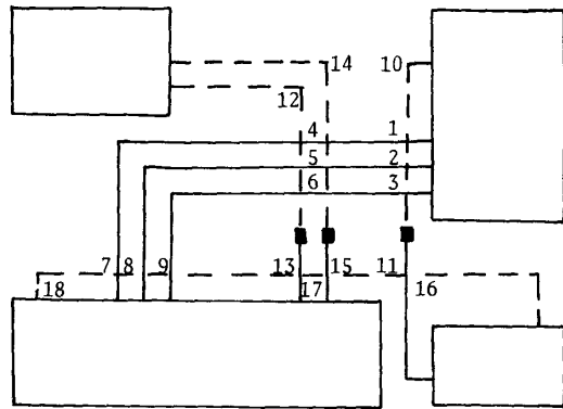
Fig. 2. A possible layer assignment
