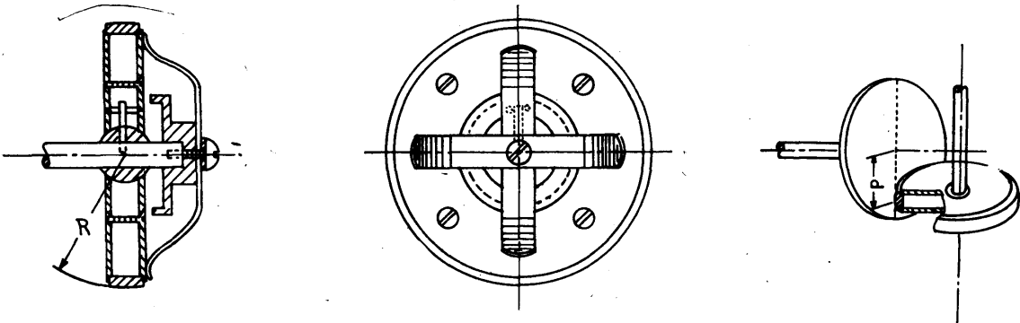
Fig. 1 - Schematic Diagram of Integrating Wheel.
