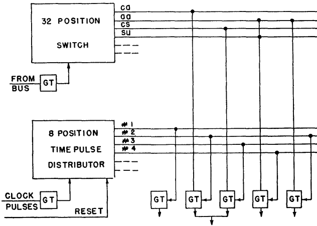
Figure 4. Operation control
