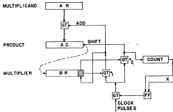
Figure 7 (above). Arithmetic element
