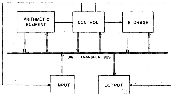
Figure 3 (right). Control
