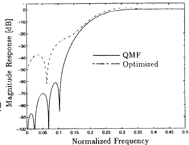
Figure 4(b): Filter Bank (High)
