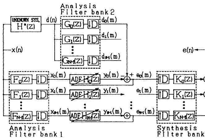
Figure 1: Subband Adaptive Filter
