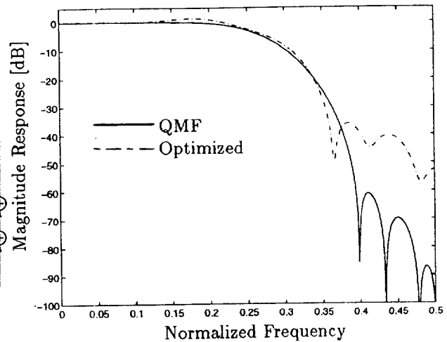
Figure 4(a): Filter Bank (Low)
