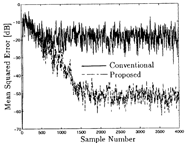
Figure 5: Learning Curves
