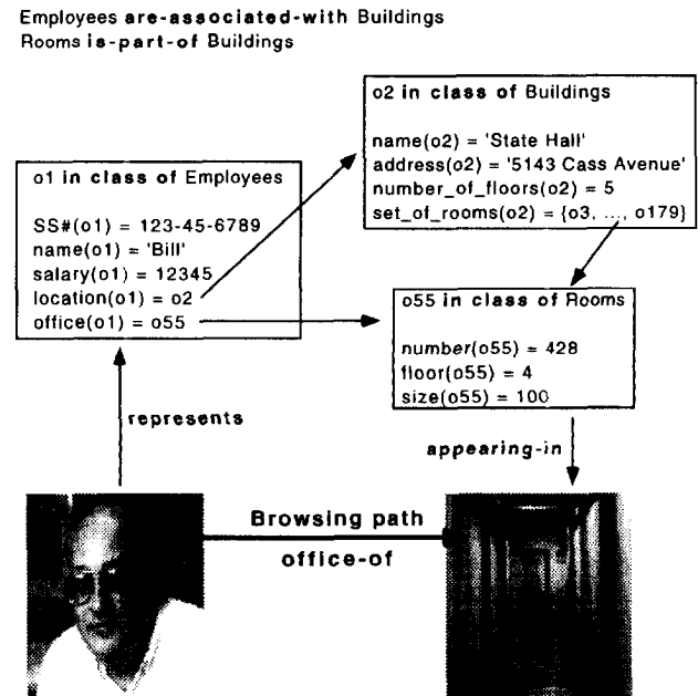
Figure 1: An Example Browsing Path Between Media Objects
