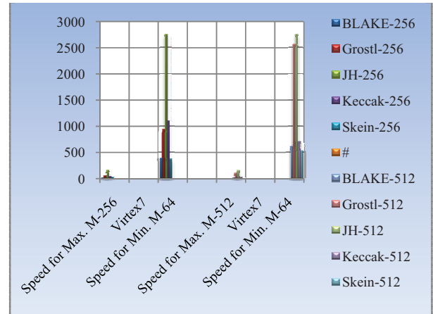
Figure 1: chart diagram for analysis speed of finalist SHA-3 in speed cycles in byte
