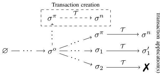
Fig. 3. Oracle-transcript based transactions can be applied in any compatible state. The transcript \mathcal{T} defines a partial function \{\sigma^\pi \mapsto \sigma^n, \sigma_1 \mapsto \sigma'_1, \dots\} .
