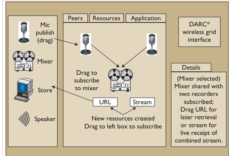
Figure 3. Example user interface for DARC*. Drag and drop allows users to easily publish their services and compose them into applications.
