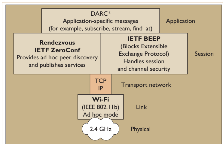
Figure 4. A full protocol stack for DARC*. The implementation architecture for this distributed audio-recording application illustrates the DARC* system.
