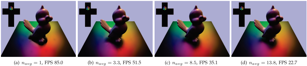
Fig. 2. Demonstration of the quality and performance trade-off, n_{avg} is the average number of cells generated per pixel.
